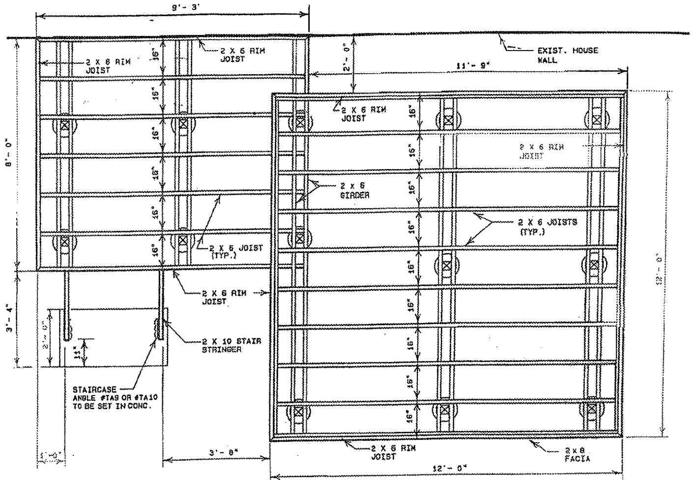
DECK FRAMING PLAN
