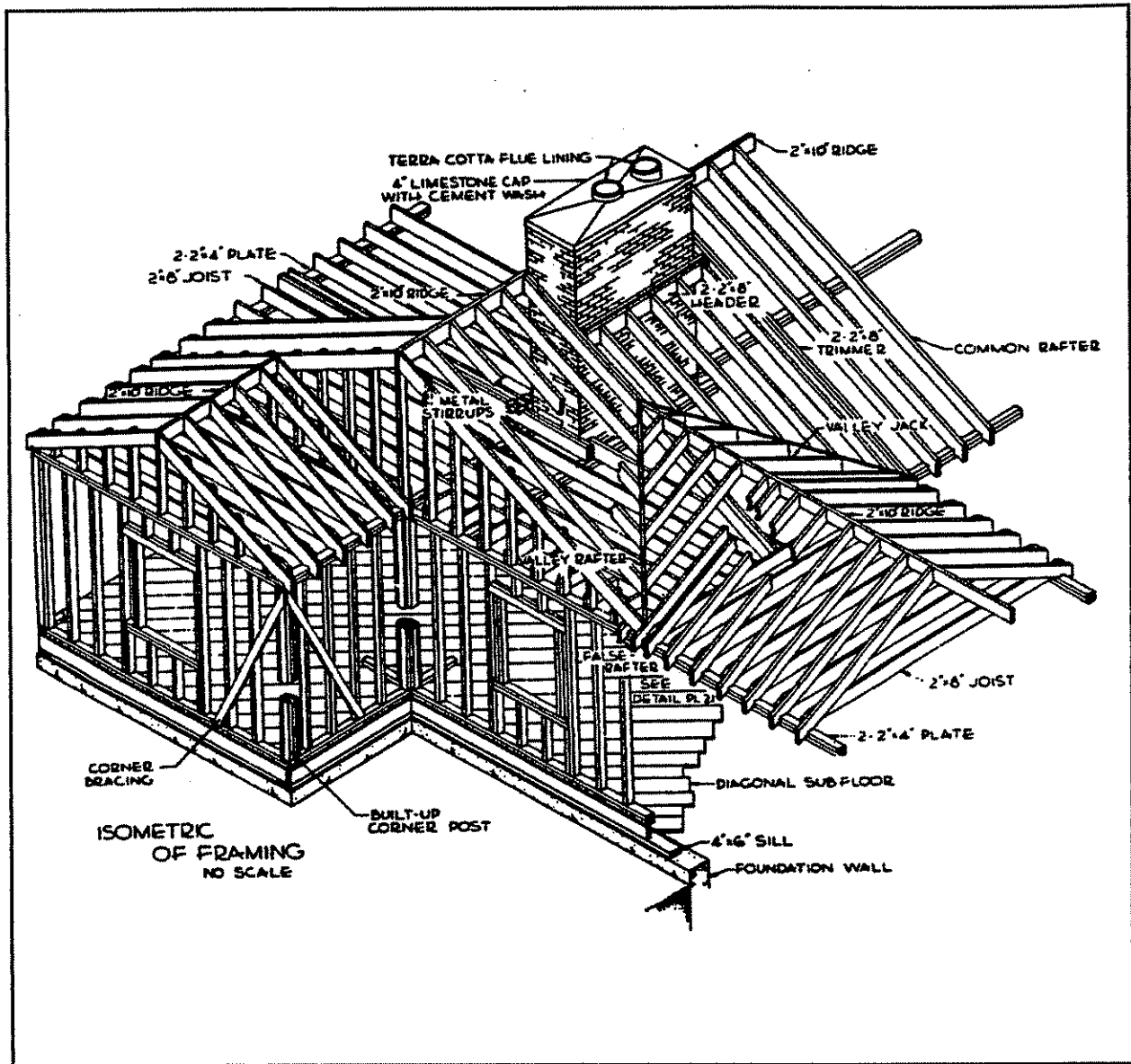
Isometric Drawing of Building Framing Figure 2-13
