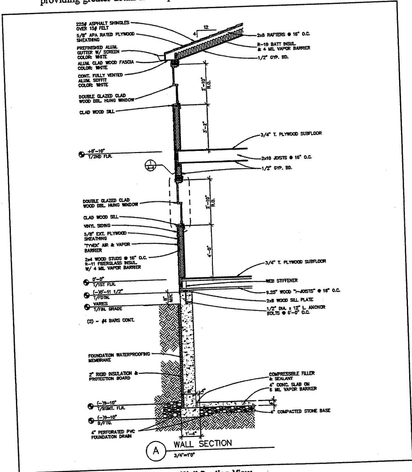
Wall Section View Figure 2-12
